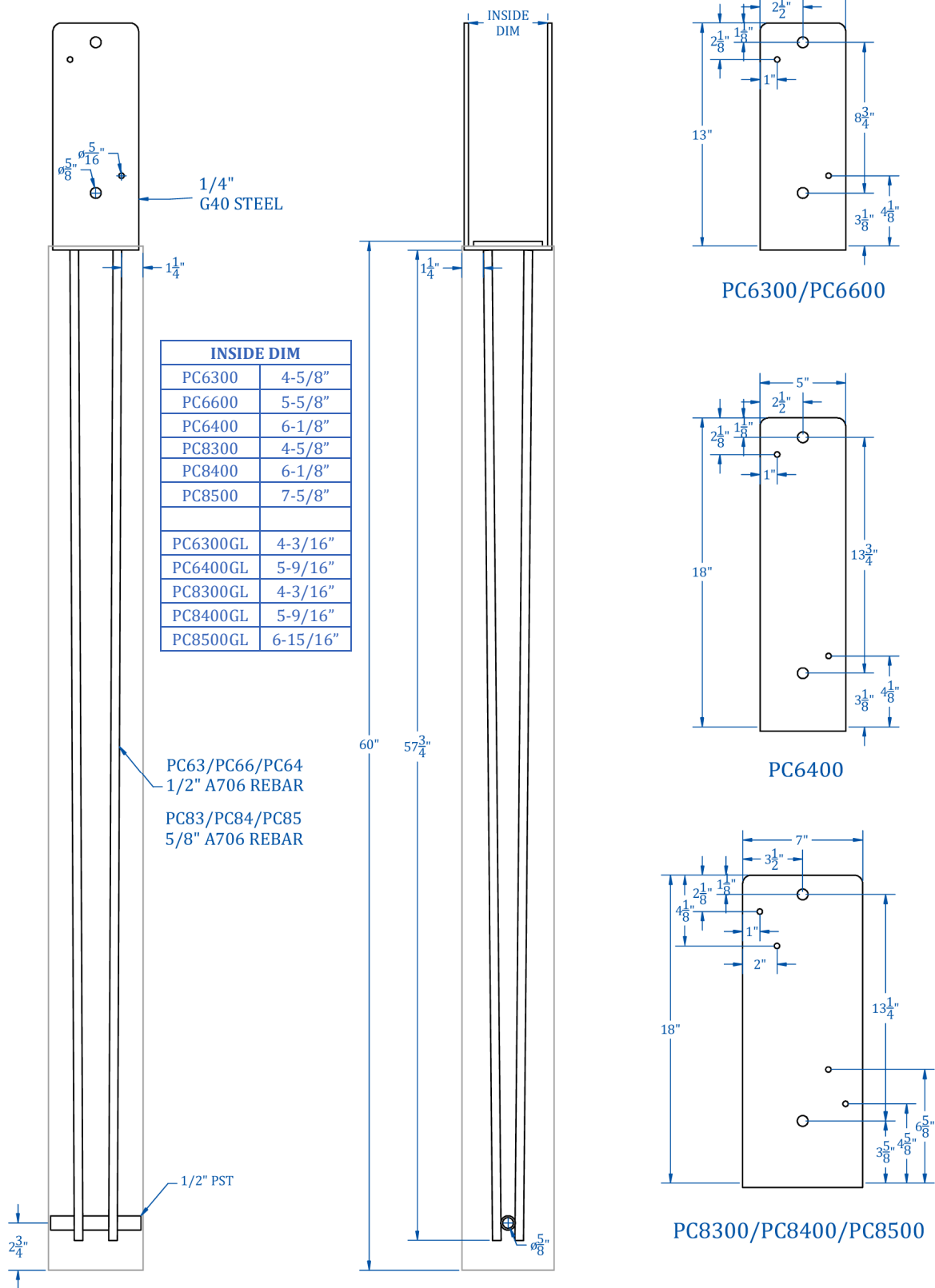
Figure 4.2 Structural Reinforcing Bracket Assemblies
